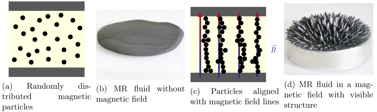
Figure 2: Behavior of MR fluids under different conditions
