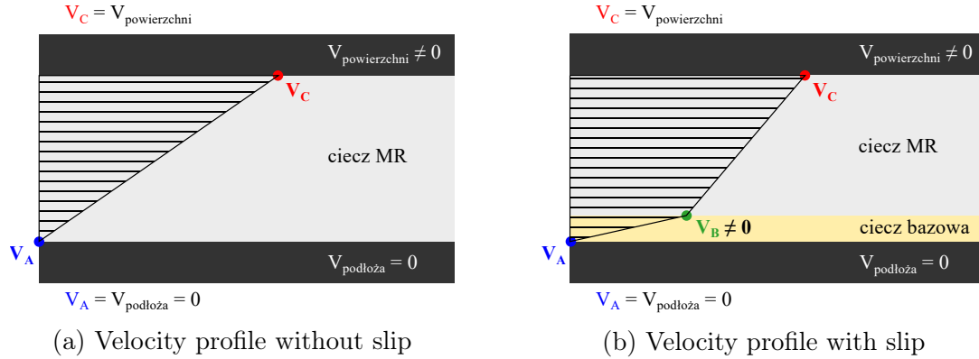
Figure 1: Liquid velocity distribution near a solid boundary
